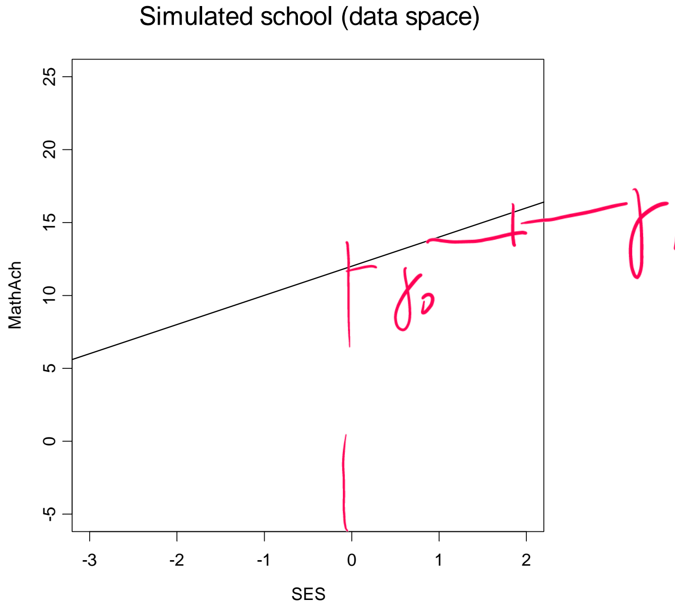
Figure 8: Simulation: mean population regression line \gamma
