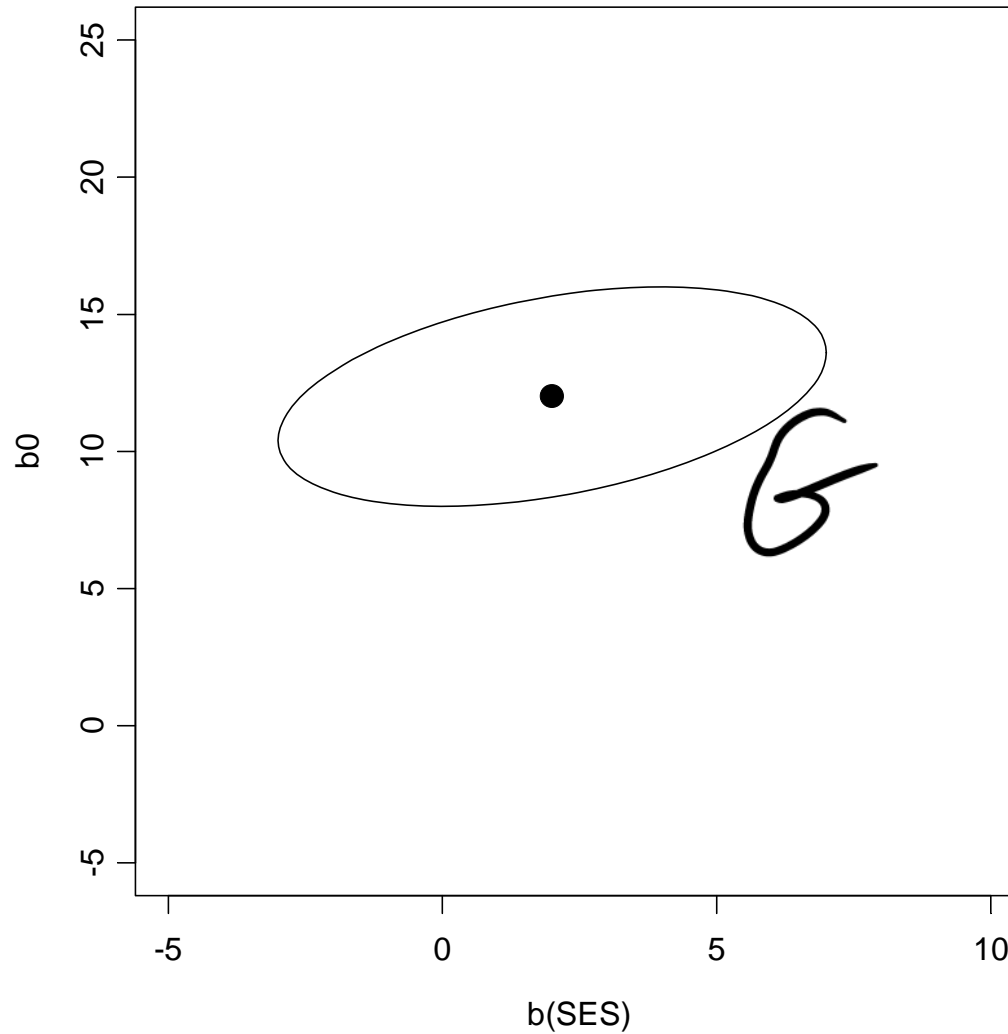
Figure 13: Simulated school: population mean line in beta space with dispersion ellipse with matrix G for random slopes and intercepts. Note that shadows of the ellipse yield the mean plus or minus 1 standard deviation
