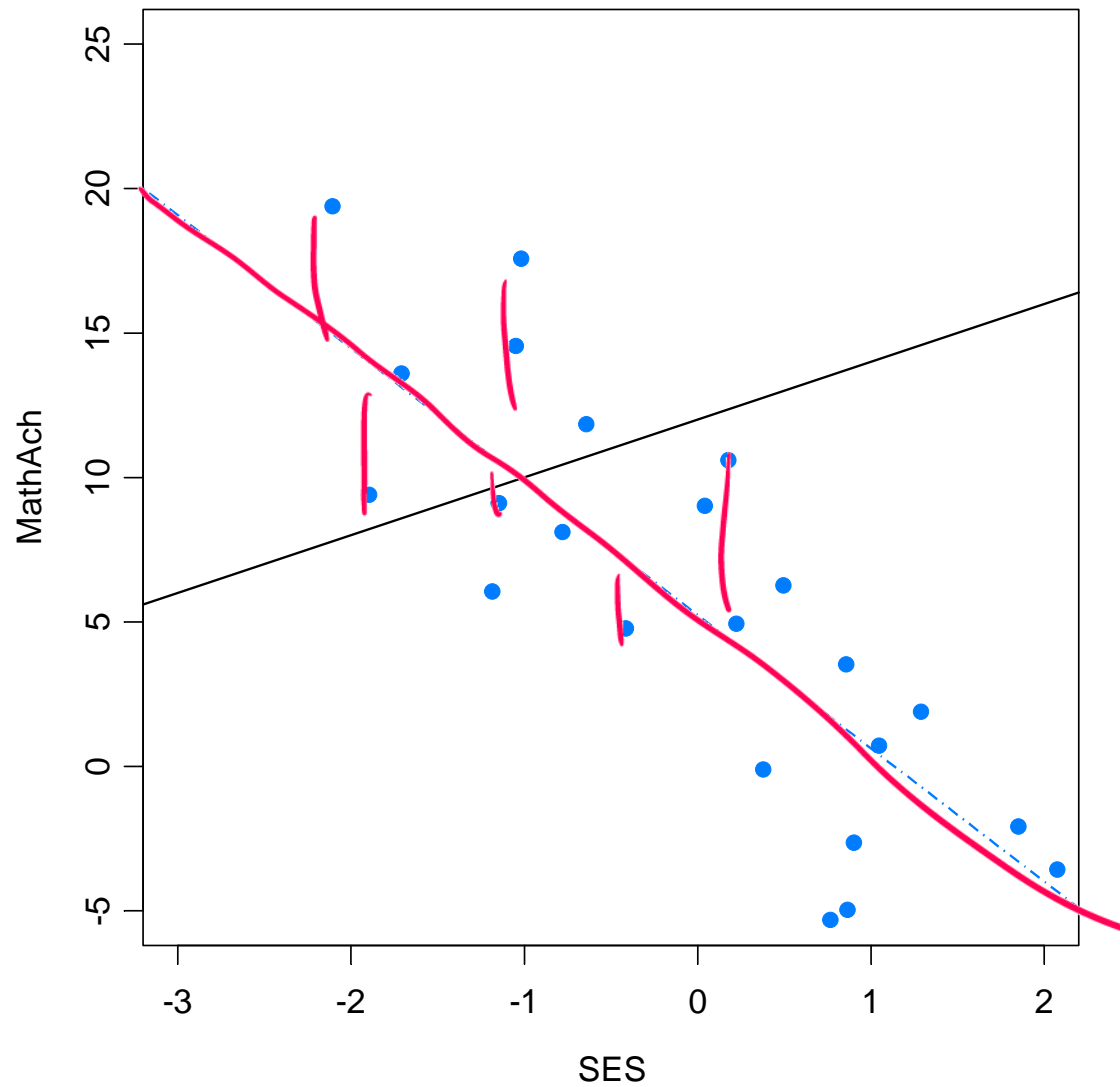
Figure 10: School 1 regression line with data generated by
