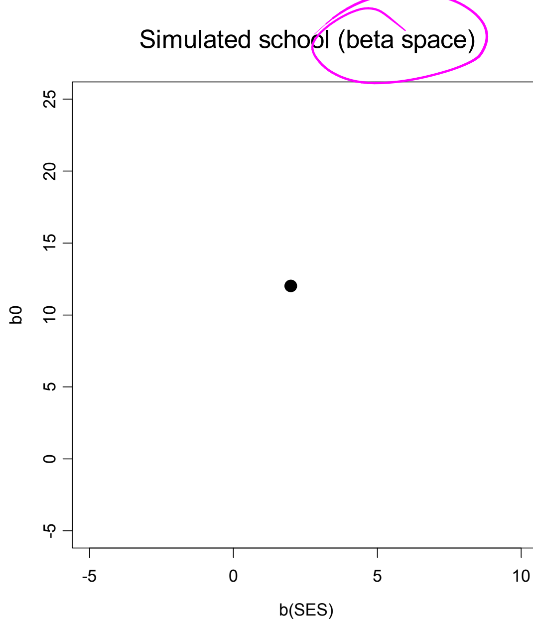
Figure 12: Simulated school in beta space with true mean line represented by a point.
