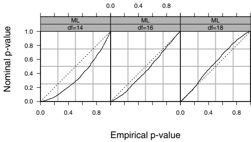
FIGURE 2.6. Plots of the nominal versus empirical p -values for the likelihood ratio test statistic comparing two models for the PBIB data. The alternative model has a fixed effect for Type , but the null model does not. The random effects specifications are the same. Both models were fit to 1000 sets of data simulated from the null model, and the likelihood ratio test statistics from the maximum likelihood estimates were calculated.
